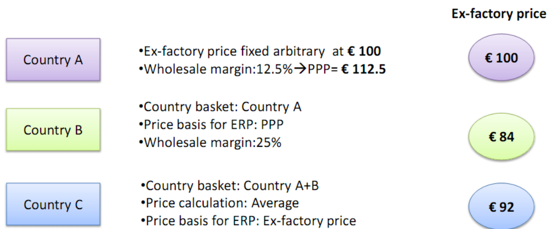
Figure 27. Illustrative representation of the margin effect
