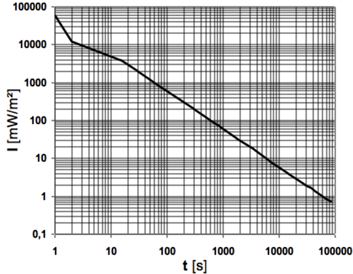
Figure 1: Recommended limits of the spectral irradiance I at 254 nm in dependence on exposure time t (ISO 15858) to reach the limit of 60 J/m 2 under constant continuous exposure during time.
