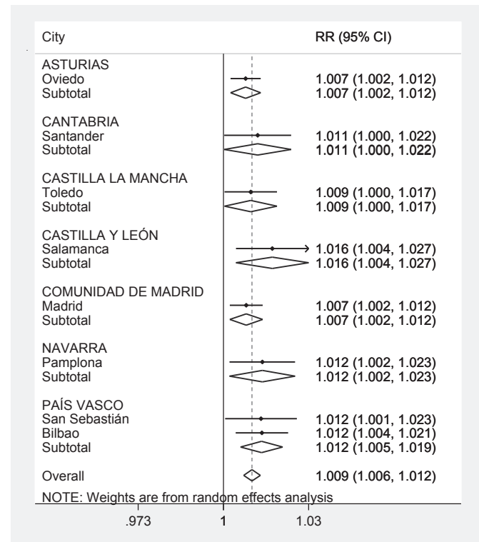
Fig. 3. Relative Risks (RR) calculated for increases of 10 \mu\text{g}/\text{m}^3 in \text{PM}_{10} levels due to circulatory causes mortality. Only showed cities with valid statistically significant associations ( p < 0.05 ) between PM and circulatory mortality causes.
